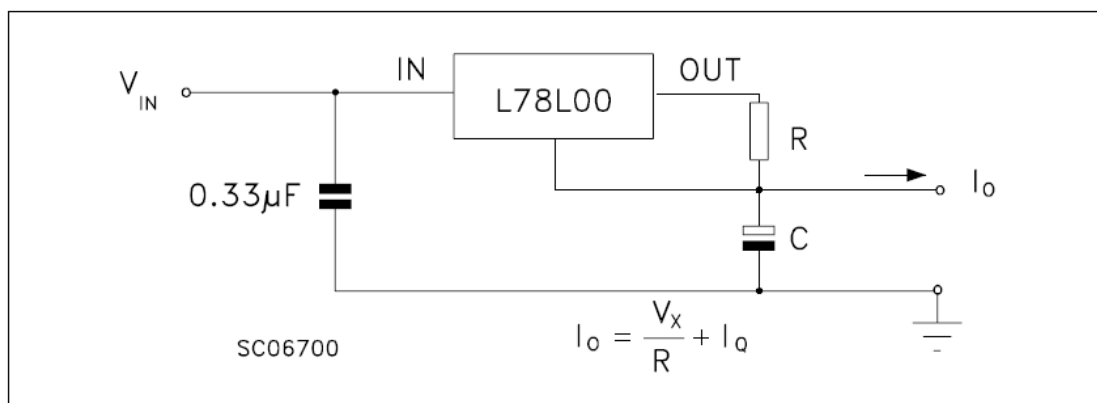
Figure3.4.15. Current regulator
