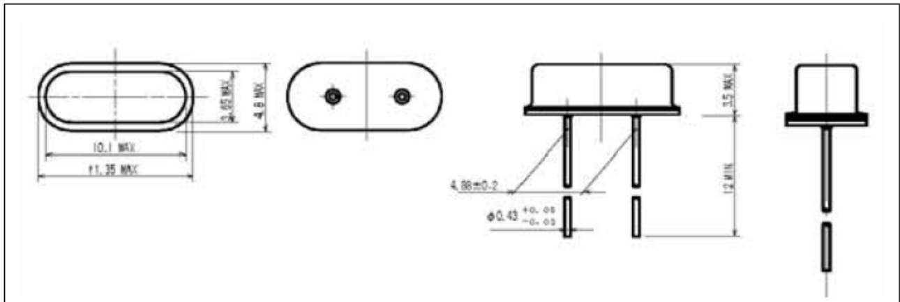
Figure3.8.1. Outline Diagram
